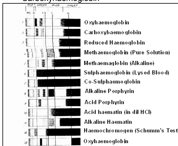
Figure 5.8: Adsorption spectra of haemoglobin and its derivatives
